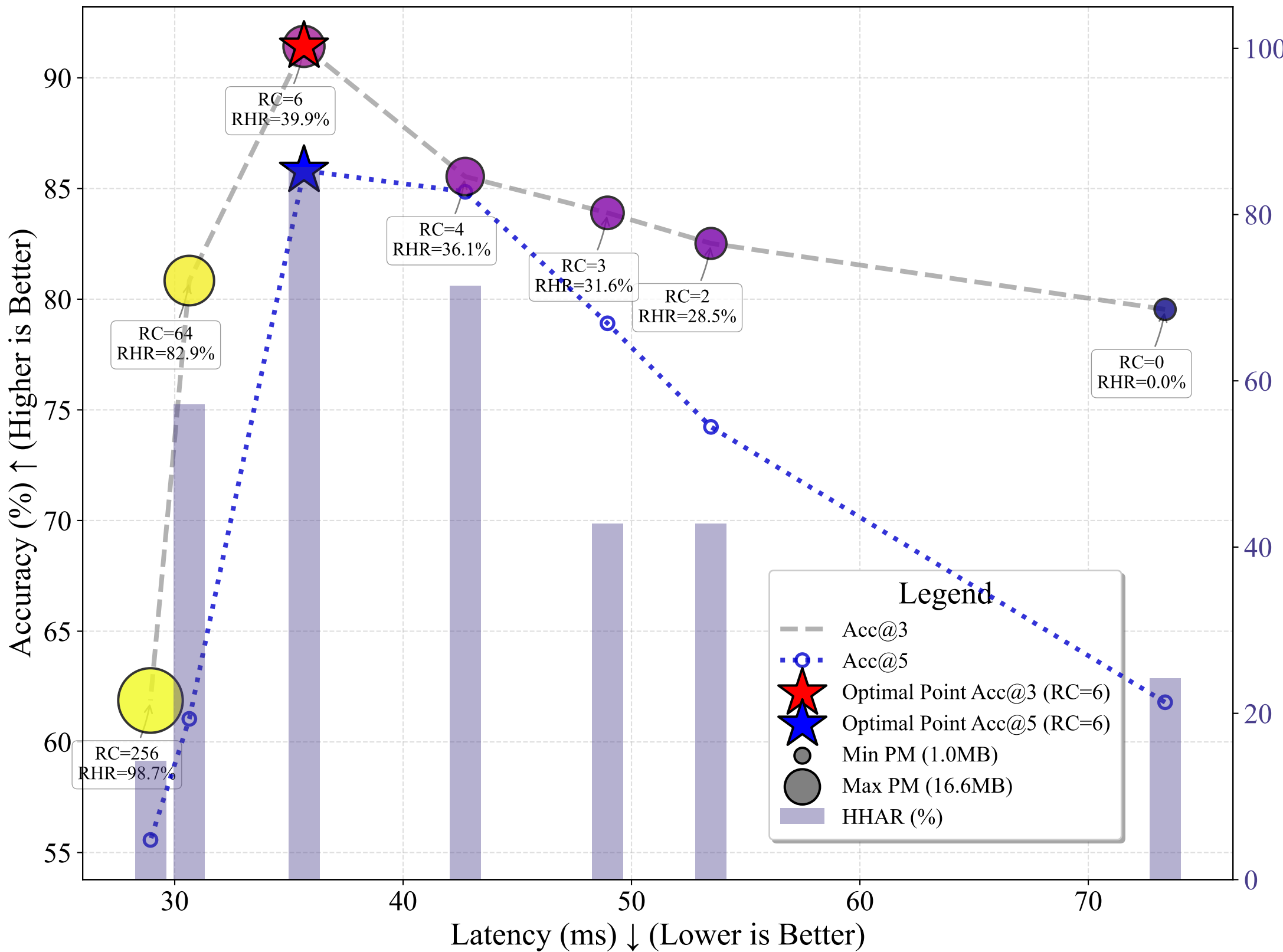
Performance Trade-off Analysis for Nba
